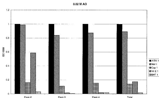
Figure 9. Comparison of antioxidant effectiveness of four antioxidants at 0.020 M concentration. Conditions as in Figure 6.
