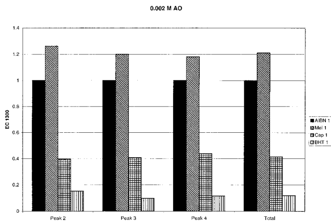
Figure 7. Comparison of antioxidant effectiveness of four antioxidants at 0.002 M concentration. Conditions as in Figure 6.
