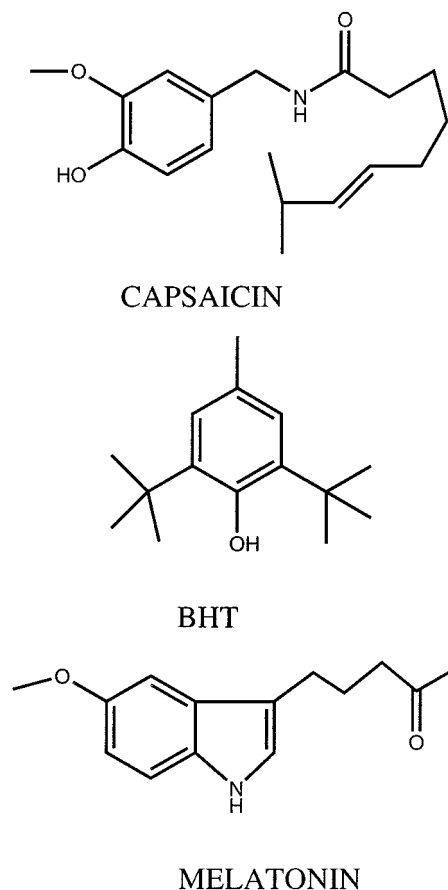
Figure 1. Structures of antioxidants.
