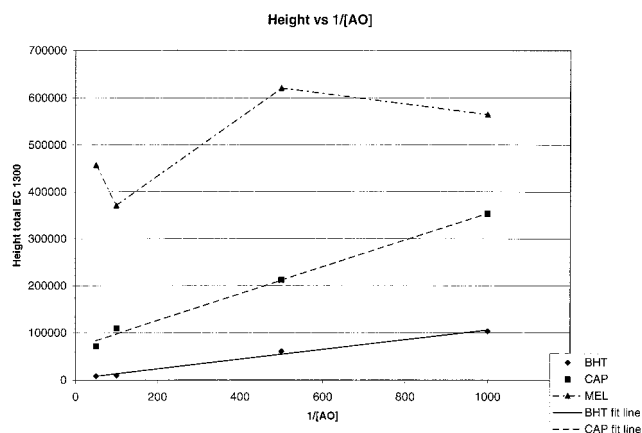
Figure 10. Plot of total lipid hydroperoxide peak height as a function of the reciprocal of antioxidant concentration. Least-squares lines for BHT and capsaicin with correlation better than 0.99. Line for melatonin shows nonlinear relationship.
