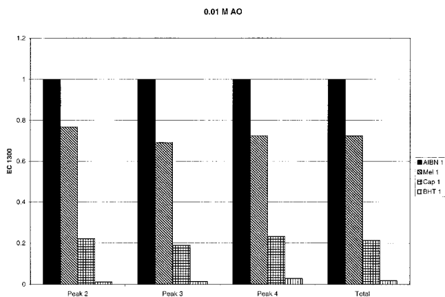
Figure 8. Comparison of antioxidant effectiveness of four antioxidants at 0.010 M concentration. Conditions as in Figure 6.
