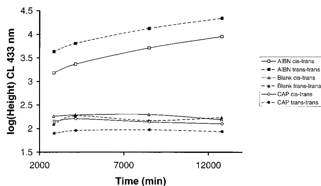
Figure 5. Comparison of the log of total cis – trans hydroperoxide peak height and the log of total trans – trans hydroperoxide peak height as a function of time. Lipid solutions as in Figure 4.
