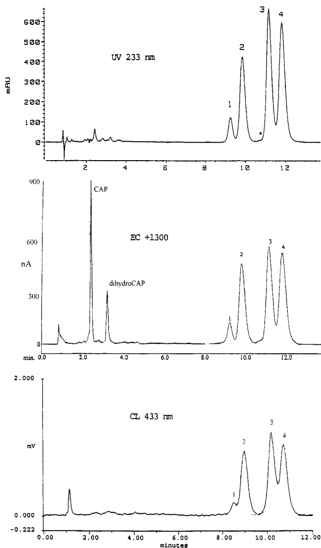
Figure 3. Chromatograms of 0.20 M linoleic acid, 0.001 M capsaicin, 0.02 M AIBN mixture after extensive lipid oxidation. Flow rate 1.3 mL/min; column temperature 50^\circ\text{C} ; mobile phase 70% methanol, 30% water, with 2% acetic acid. For EC and UV detection, mobile phase was also 0.030 M in tetraethylammonium perchlorate. Chemiluminescence luminol solution added postcolumn at 3.0 mL/min. Peaks between 2 and 4 min in EC chromatogram are capsaicin and dihydrocapsaicin. Hydroperoxide peaks identified in text. Asterisk (*) indicates the position of peak 5.
