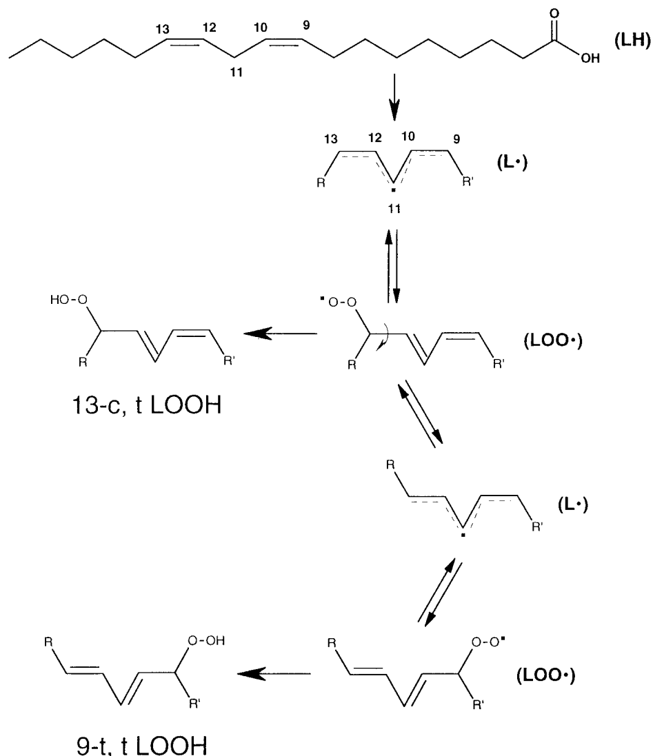
Figure 2. Partial mechanism of oxidation of linoleic acid (Adapted from Porter, 1984).
