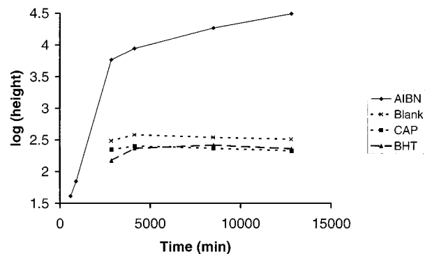
Figure 4. Time series plot of the log of total lipid hydroperoxide peak height (peaks 2–4) using chemiluminescence detector. Solutions 0.20 M lipid, 0.020 M AIBN, and 0.020 M antioxidant in air.
