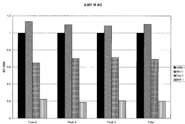
Figure 6. Comparison of antioxidant effectiveness of four antioxidants at 0.001 M concentration. Data from electrochemical detector at 1300 mV. All peak heights normalized to 0.020 M AIBN solution and 0.20 M linoleic acid in air without antioxidant. Oxidation at 30 °C for 8 days.
